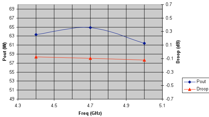
IG4450M50 Pout & Droop vs Freq 300 \mu\text{s} , 10%, 40V, 40mA
