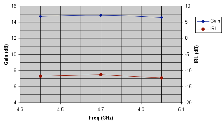
IG4450M50 Gain & IRL 300 \mu\text{s} , 10%, 40V, 40mA
